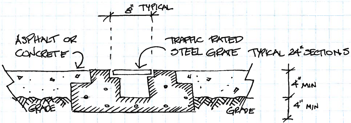
SECTION THRU SITE BUILT DRIVEWAY TRENCH DRAIN
